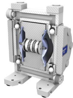
ChemSafe Models: 205, 307
